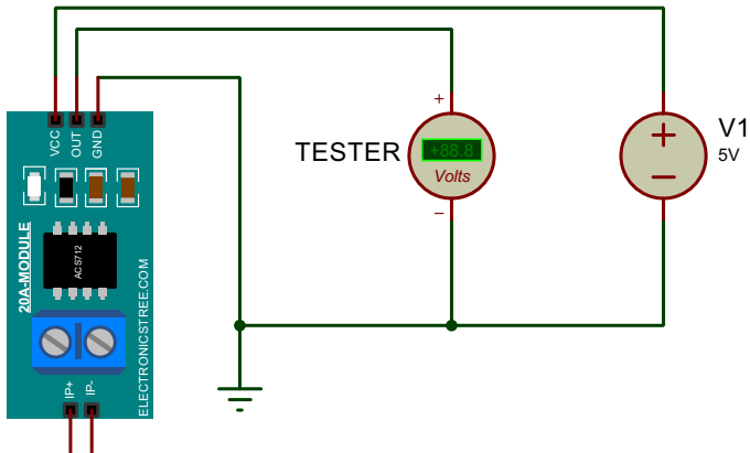
CSM1 CURRENT SENSOR 20A
